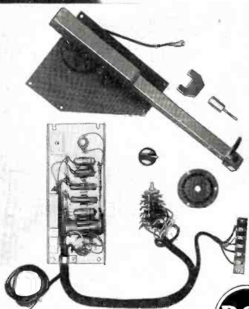
The complete Universal Pick-up Kit MI-4875-G.
